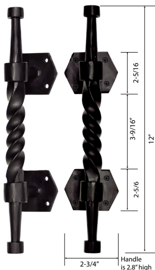
2.8 lbs Tucson Wrought Iron Pull Handle
