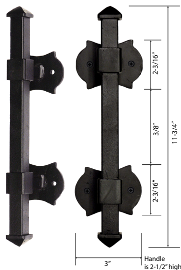
3.1 lbs San Juan Wrought Iron Pull Handle
